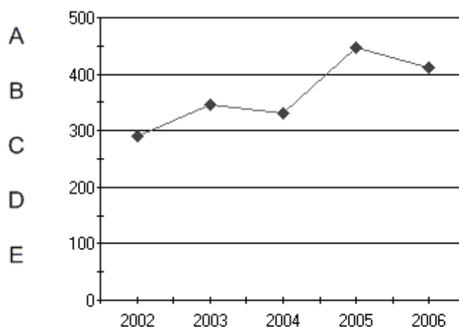
Scoring
